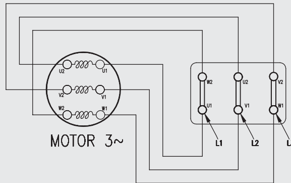
DELTA CONNECTION
