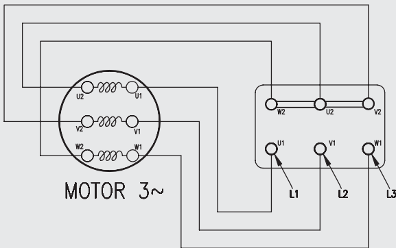
STAR CONNECTION
