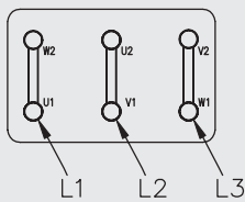
DELTA CONNECTION 400 V
