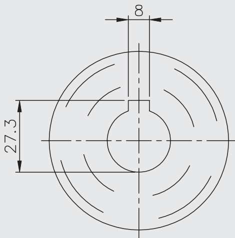
PUMP SIDE
