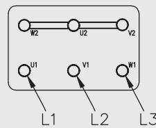
STAR CONNECTION 690 V
